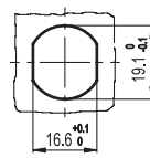
Drilling template
