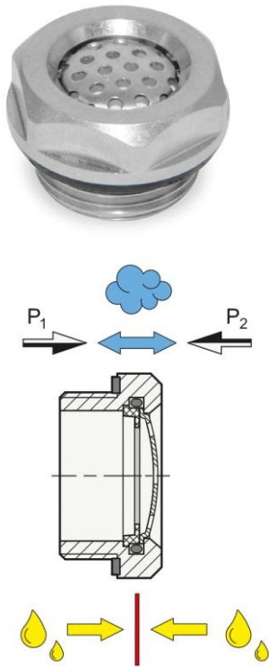
Two-way breathable membranes GN 7404
